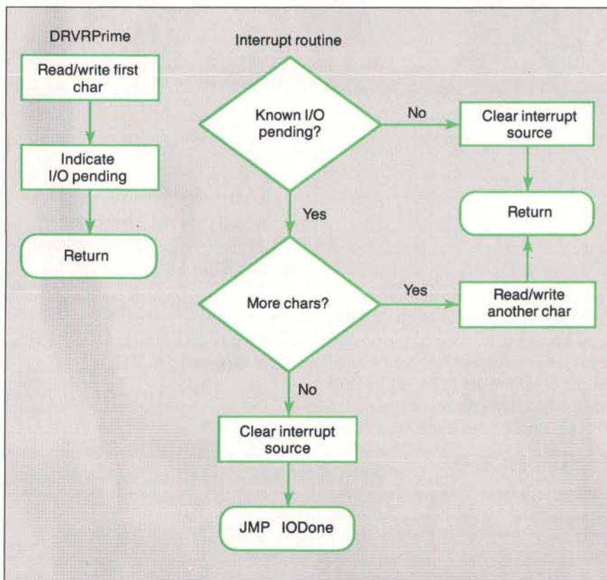
Figure 4: Flowchart illustrating read- and write-completion logic.
